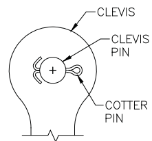
Diagram 2C. Installing cotter pin through clevis pin.
