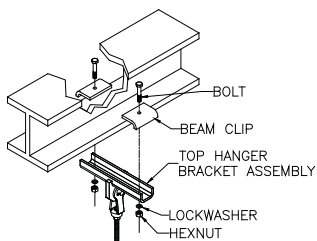
Diagram 2E. Bolting standard top hanger bracket and beam clips to existing support beam.
